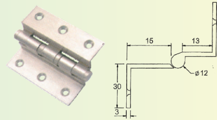
100 mm R-HINGE
